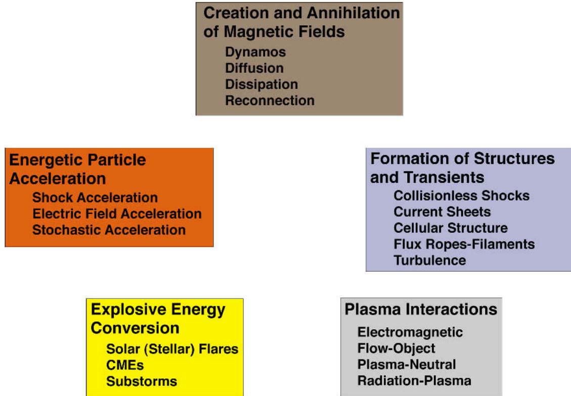
FIGURE 1.1 Five fundamental behaviors characteristic of magnetized cosmic plasmas.
