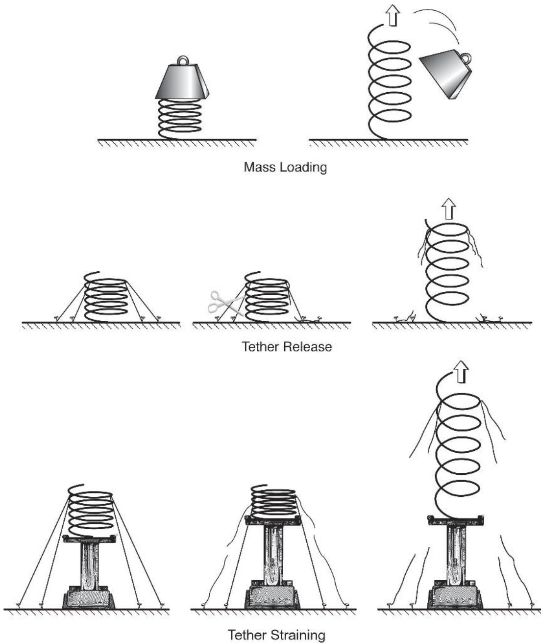
FIGURE 5.2 Three classes of coronal mass ejection models. Image courtesy of J. Klimchuk (Naval Research Laboratory). Reprinted, with permission, from J.A. Klimchuk, Theory of coronal mass ejections, pp. 143-157 in Space Weather , Geophysical Monograph 125, P. Song, H.J. Singer, and G.L. Siscoe, eds., American Geophysical Union, Washington, D.C., 2000. Copyright 2000, American Geophysical Union.
