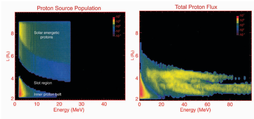
FIGURE 6.2 Computer simulation of the formation of a new proton belt during the magnetic storm of March 24, 1991. The panel on the left shows the seed population of solar energetic protons, while the panel on the right shows the new proton belt formed in the slot region as a result of the interaction of the CME-driven interplanetary shock with Earth's magnetosphere. Image courtesy of M.K. Hudson (Dartmouth University). Modified and reprinted, with permission, from M.K. Hudson, Simulations of radiation belt formations during storm sudden commencements, Journal of Geophysical Research 102(A7), 14087-14102, 1997. Copyright 1997, American Geophysical Union.
